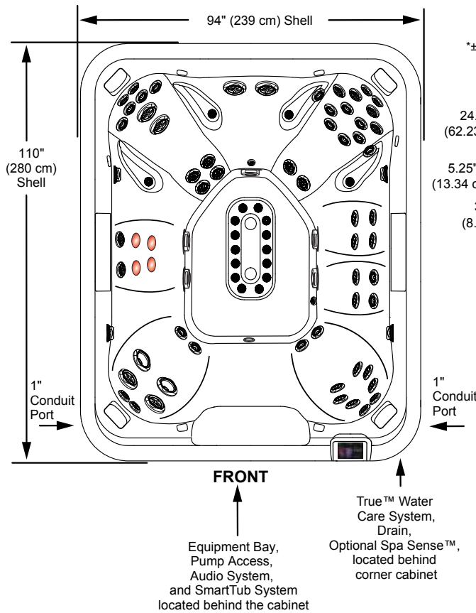
TOP VIEW
